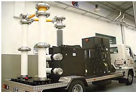
Truck produced by Inducor from Argentina with VLF-200CMF and generator. Partial Discharge and Tan Delta diagnostic cable testing products are provided by Power Diagnostix from Germany. Picture to the right is basic VLF-200CMF model.
