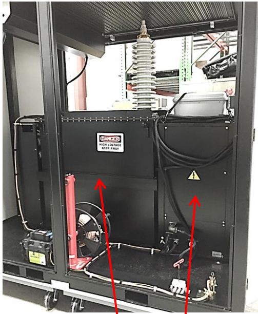
Side view showing HV tank & Regulator sections Battery & ground cable reel with 30' (10 m) #2 AWG
