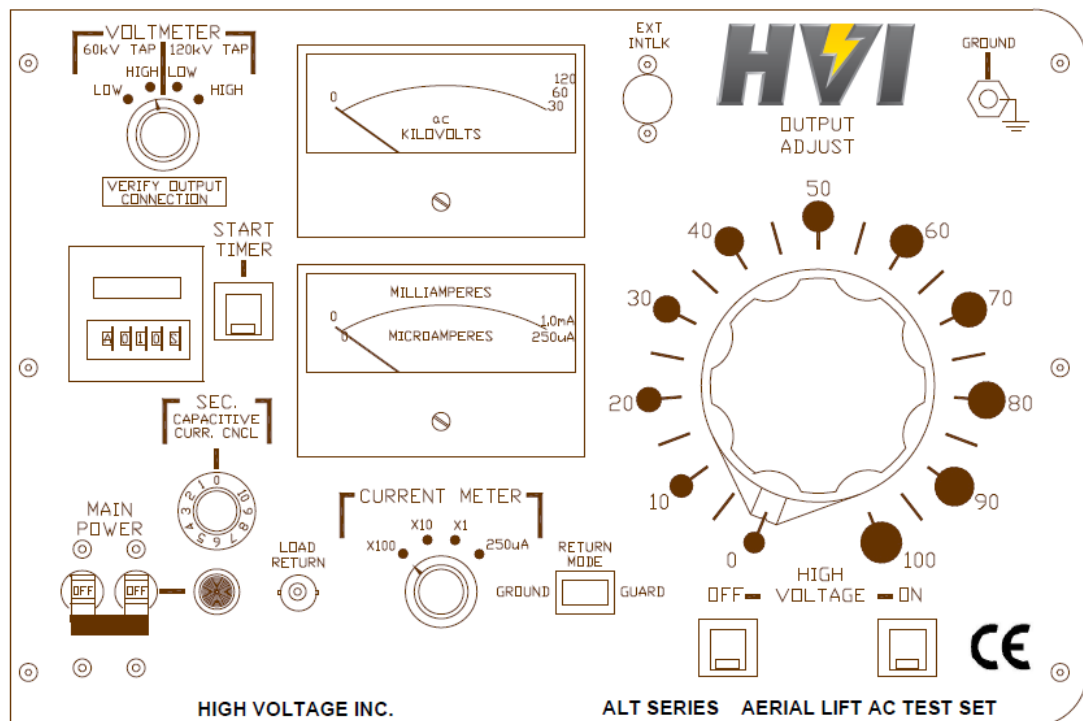
Figure 1 ALT-120/60FCC front panel controls.
