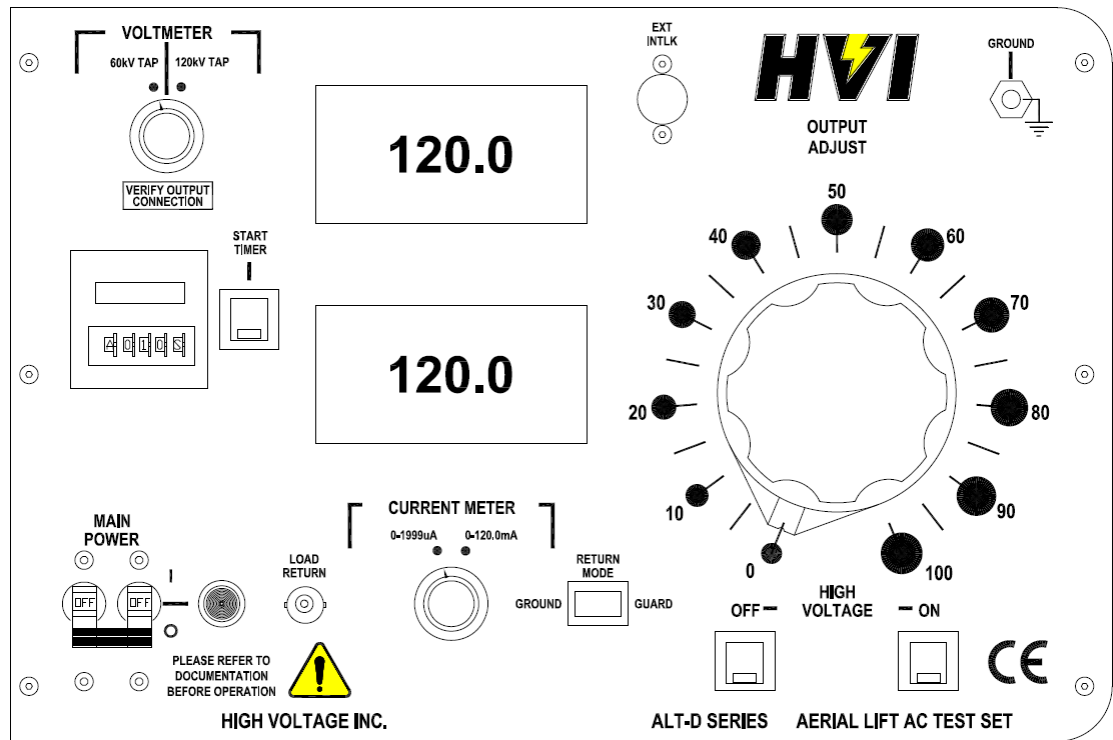
Figure 1 ALT-D Series front panel controls.
