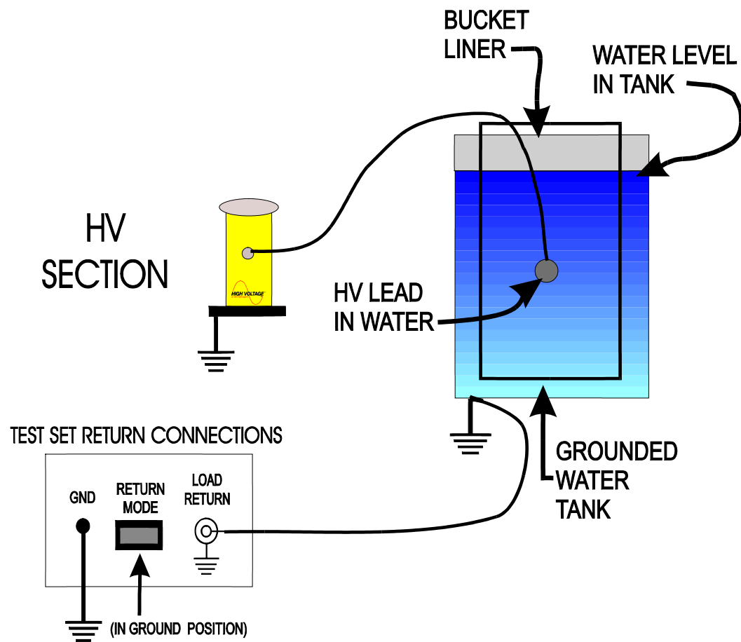
FLASHOVER TEST ON BUCKET LINER IN WATER
