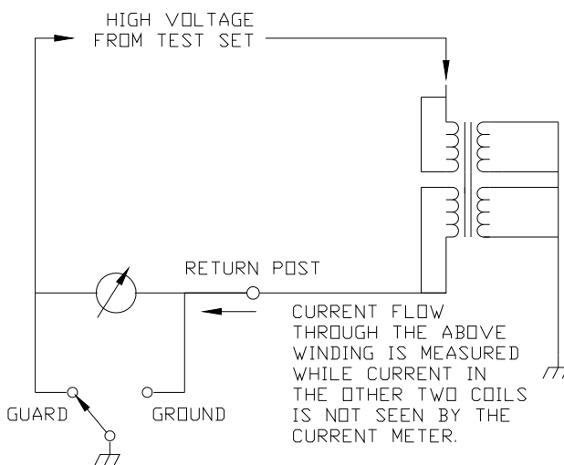
Figure 3, Guarded Return Diagram
