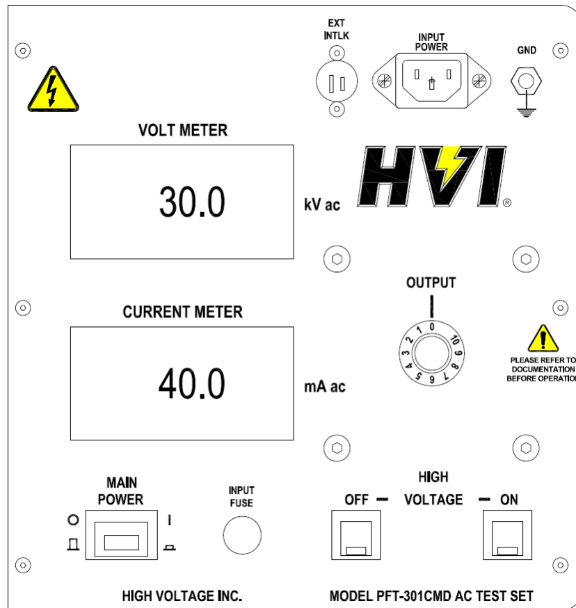
Figure 1 PFT –301CMD front panel controls.
