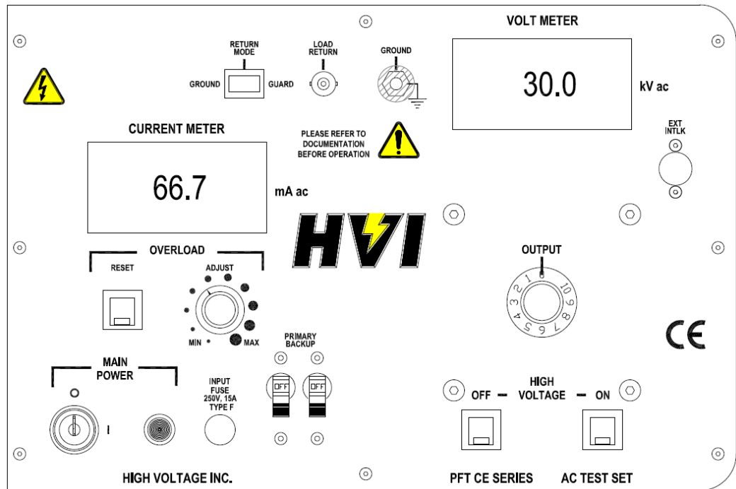
Figure 1 PFT-302CE front panel controls.
