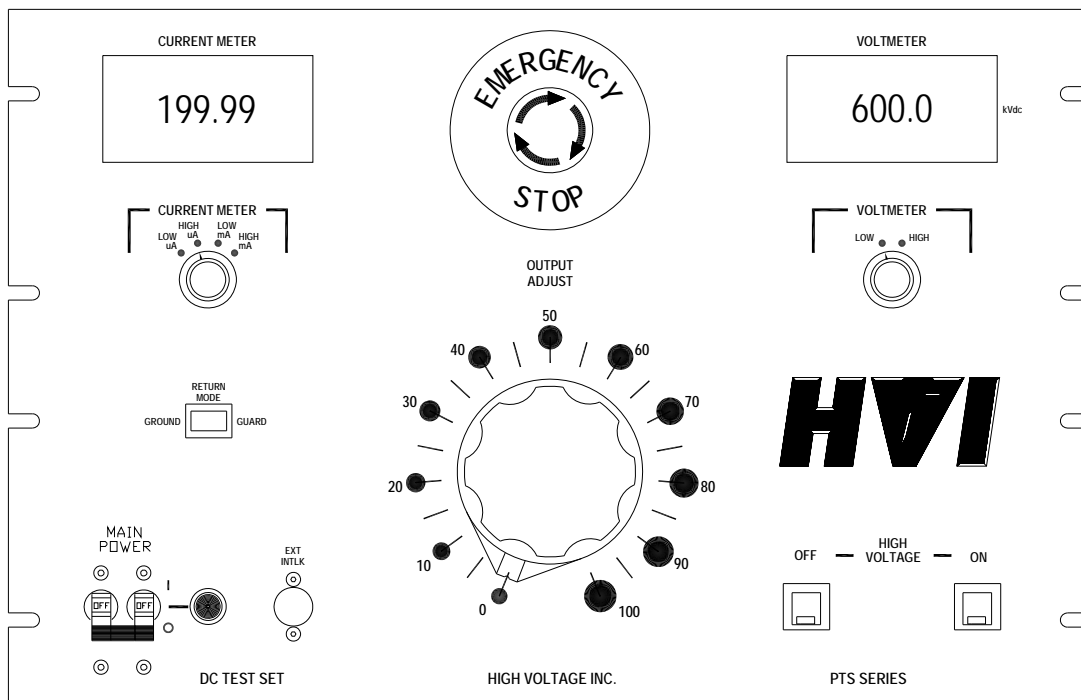
Figure 2 PTS-600FBTD Series front panel controls.
