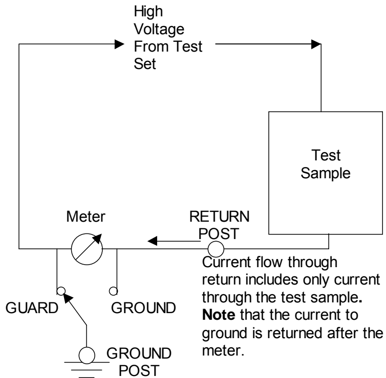
Figure 3, Guarded Return Diagram
