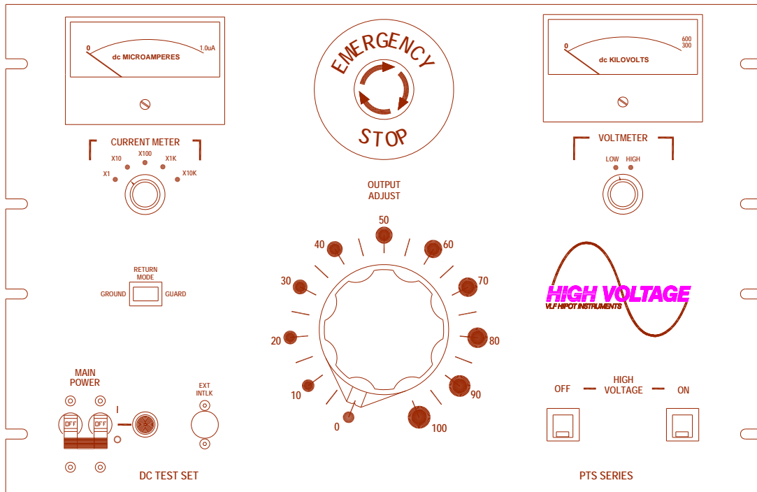
Figure 1 PTS-600FBT Series front panel controls.
