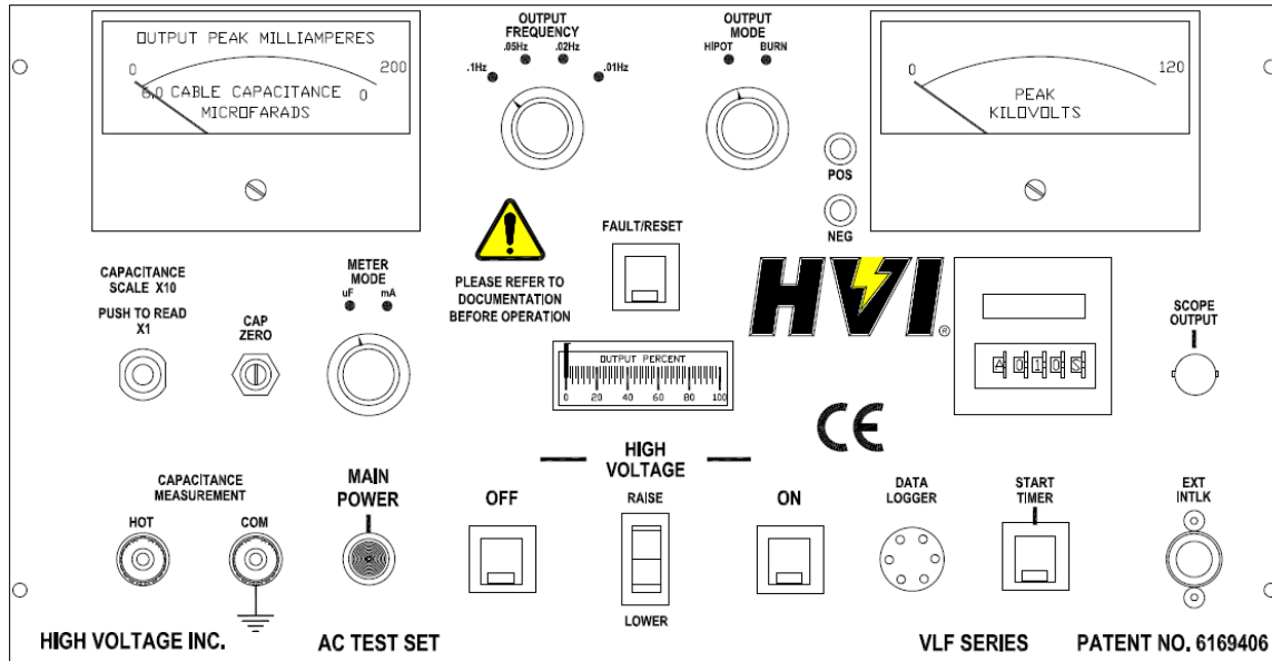
Figure 1 VLF Series front panel controls.
