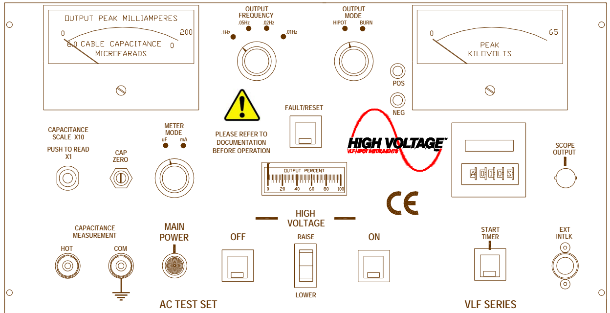
Figure 1 VLF/BURNER Series front panel controls.
